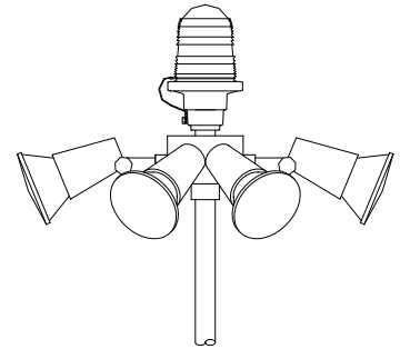
LIGHTING ASSEMBLY 6 FLOODLIGHTS AIMING ANGLE IS FACTORY PRESET
